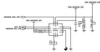
Sensor Hub integrated Accel Sensor
